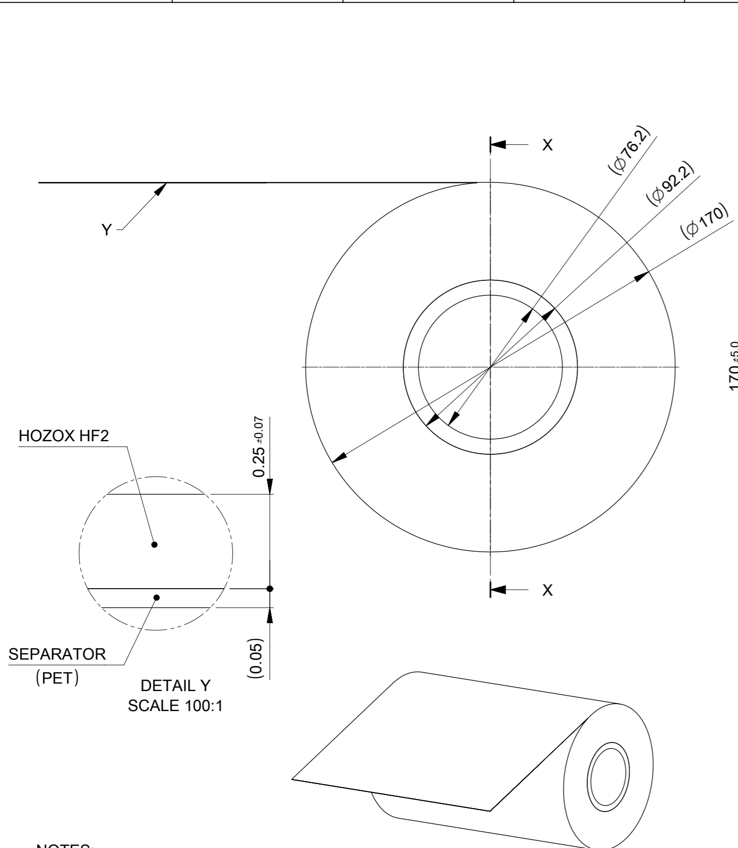
PERSPECTIVE VIEW SCALE 1:5
